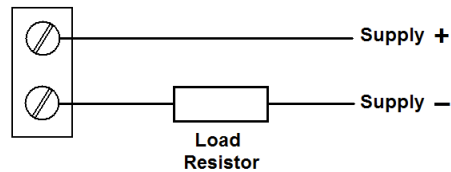
Voltage Measurement
